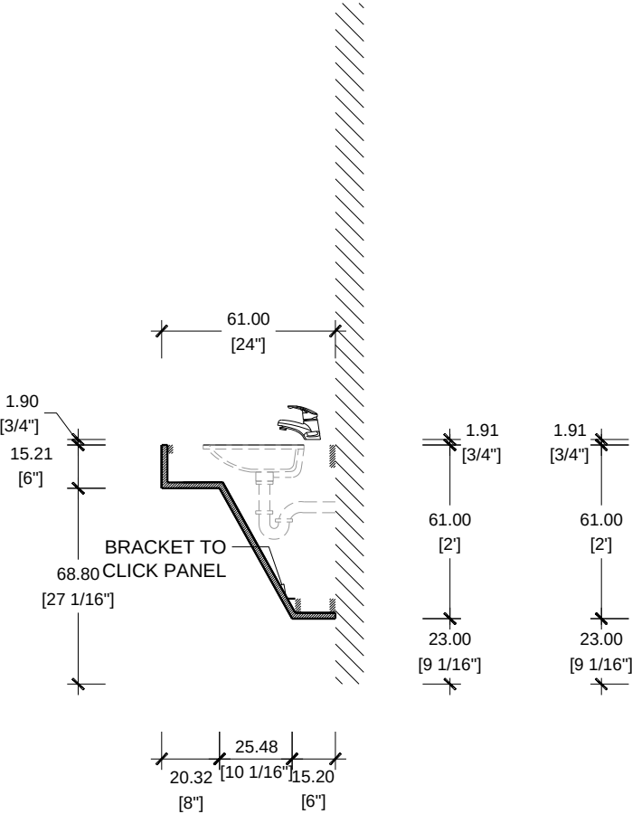
SECTION SCALE 1/2"=1'-0" CASA FAMILIA / VANITY TYPE RV2
