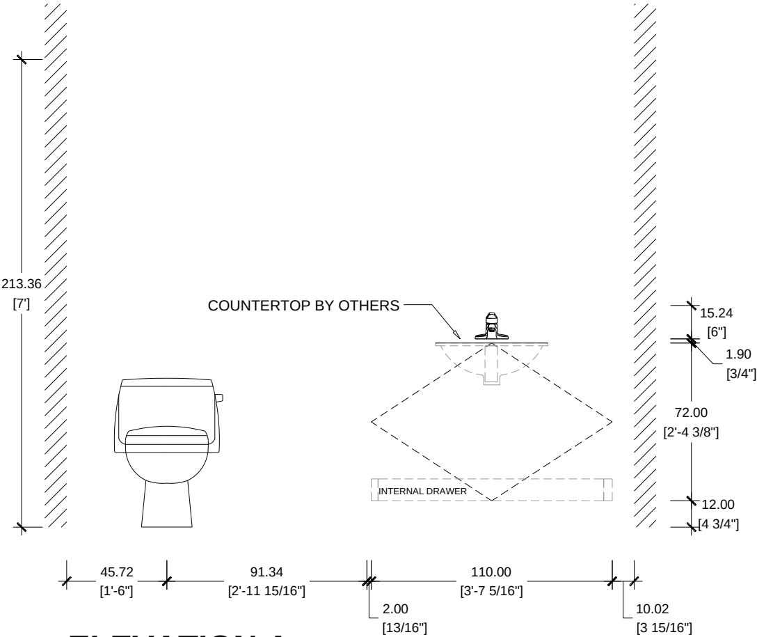
ELEVATION A CASA FAMILIA UNIT B1 / VANITY TYPE V4
