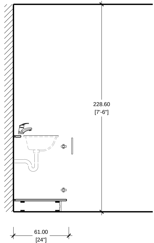
SECTION SCALE 1/2"=1'-0" VANITY
