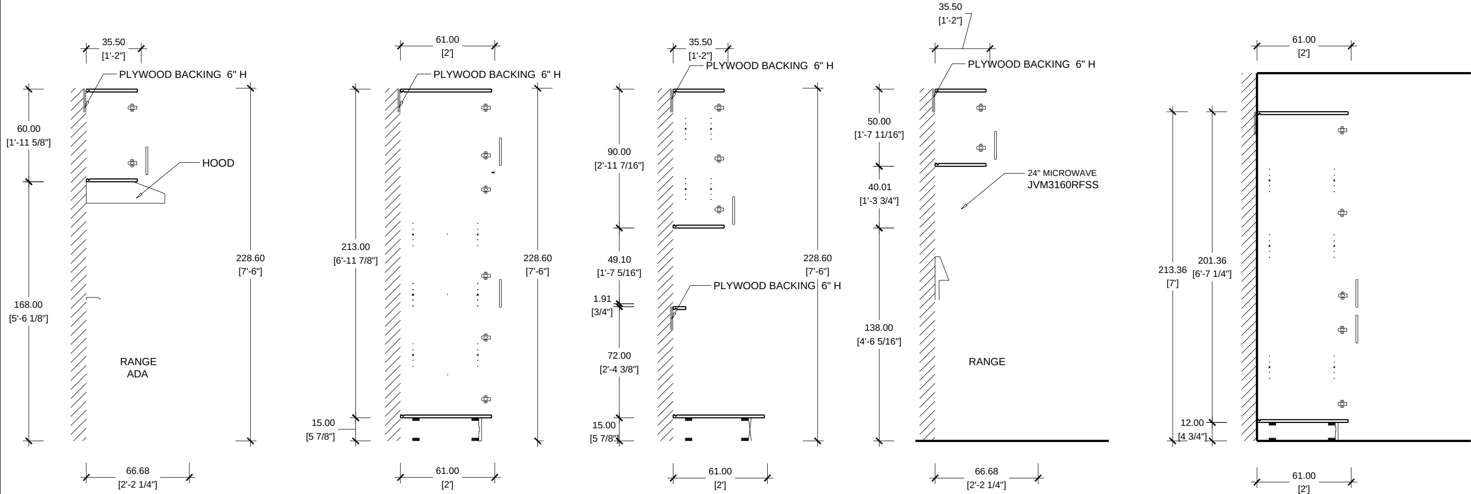
SECTION HOOD KITCHEN ADA SCALE 1/2"=1'-0"
